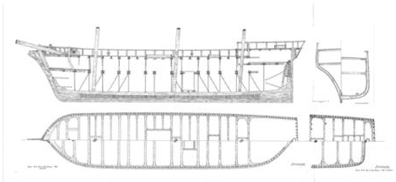
Jhelum structural plan (John Kearon)
